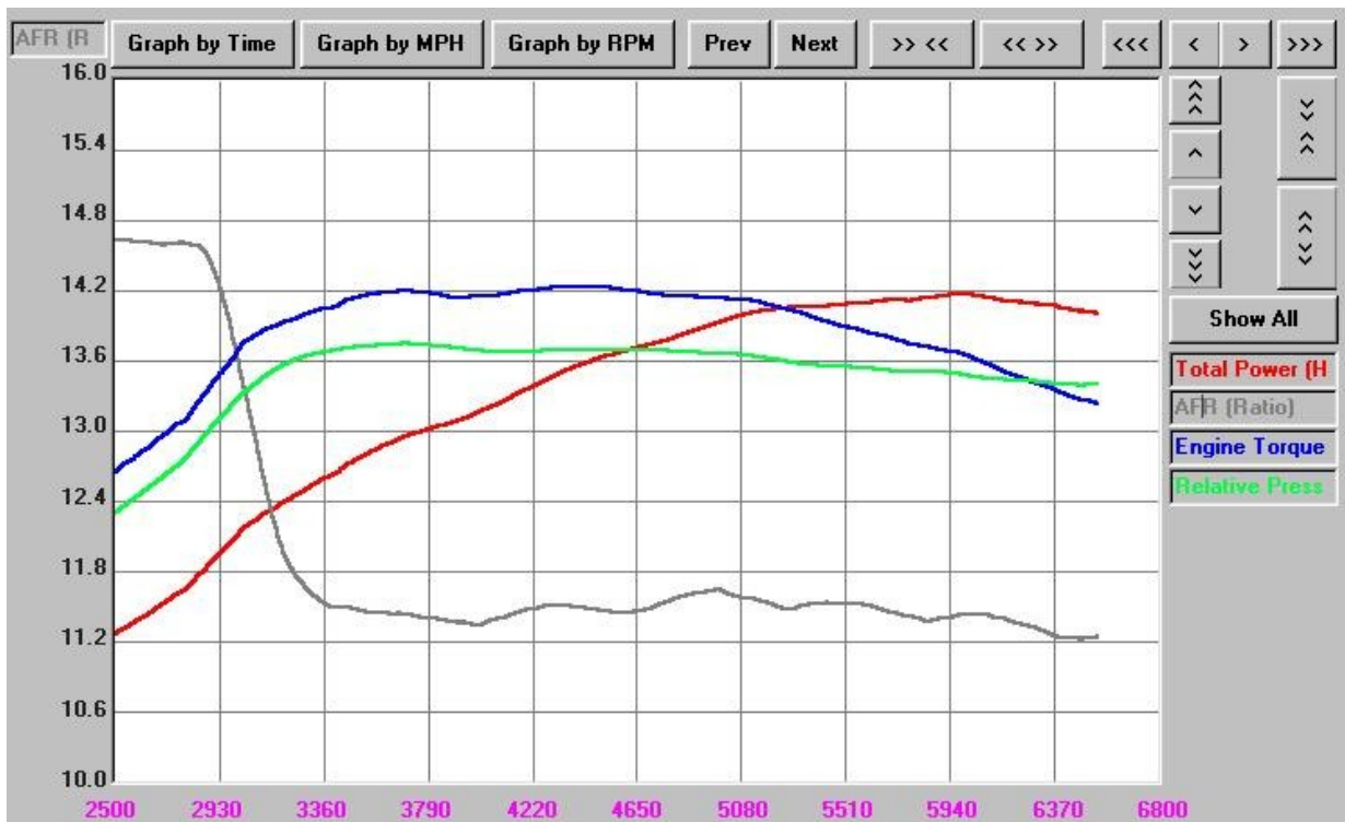
Measured Wheel Torque = blue, calculated wheel HP = red, measured relative pressure (boost) = green, grey = measured AFR Dyno Graph* A = Stage1 91 v101 with Relative Pressure Tracing
